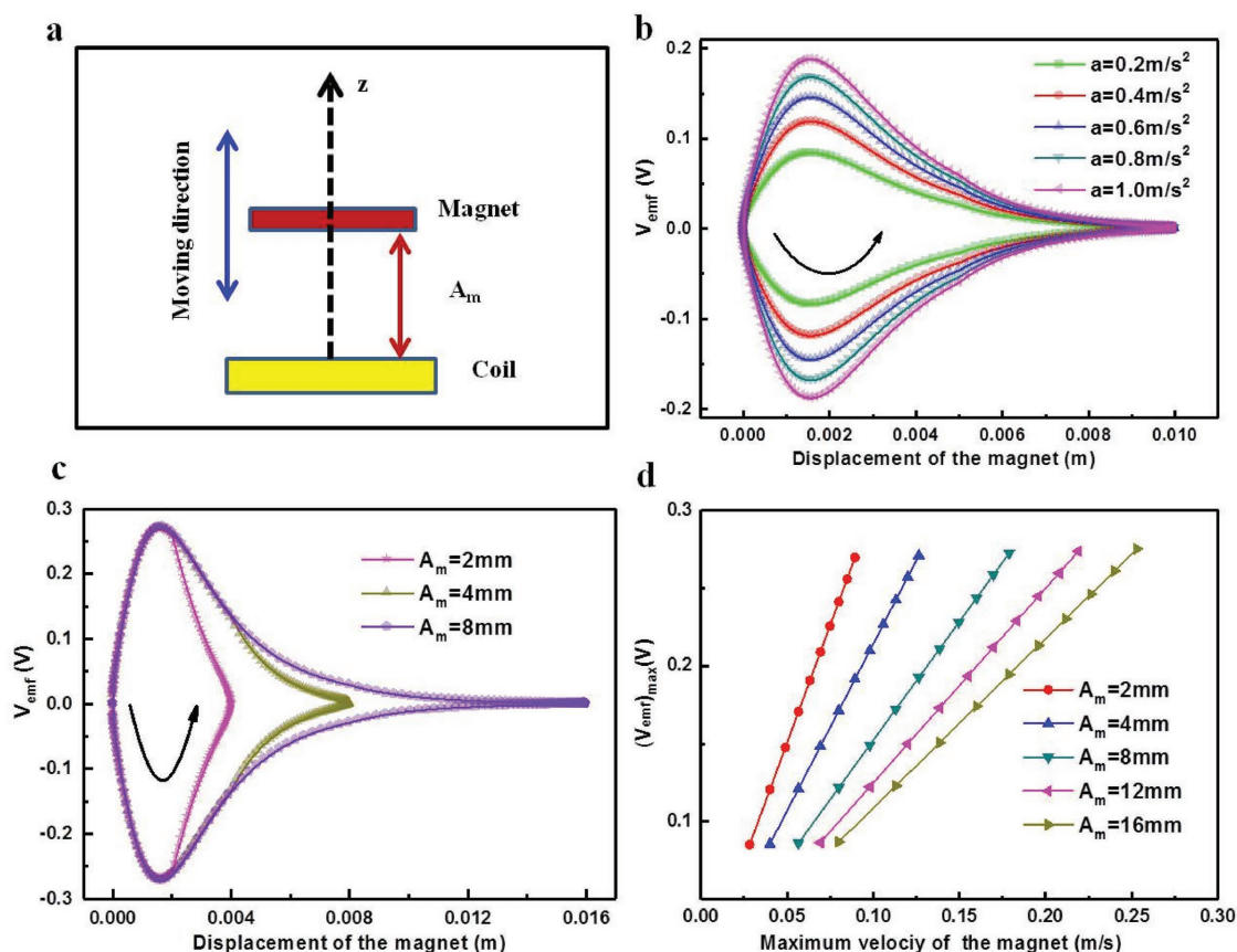
Figure 3. Theoretical calculation results of EMG. a) The schematic of magnet's movement ( A_m means the amplitude of the magnet). b) The value of V_{emf} versus the displacement and the acceleration of the magnet when A_m = 5 mm. c) The value of V_{emf} versus the displacement and the amplitude of the magnet when a = 2 m s -2 . d) The maximum value of V_{emf} versus the maximum velocity and the amplitude of the magnet.
