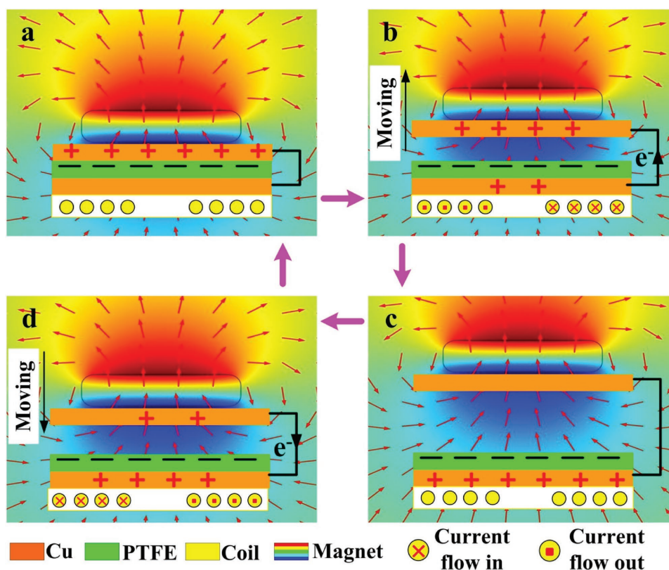
Figure 2. Schematic of the operation principle of the hybridized sensor. When the magnet is moved up and down by external force, both the TENG and EMG can generate the output voltage and current signals. A 2D axisymmetric model of the magnet was established, and the distribution of the magnetic scalar potential and the magnetic flux density were calculated by COMSOL and shown by different color and red arrows, respectively.
