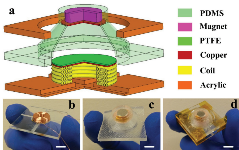
Figure 1. Structure design of the hybridized EMG-TENG active sensor. a) Schematic illustration of the multilayer structure of the hybridized sensor. b) The optical photograph of the Cu coil on the acrylic substrate (scale bar: 5 mm). c) The optical photograph of the PDMS button structure (scale bar: 5 mm). d) The optical photograph of the assembled hybridized sensor with a volume of about 25 \times 25 \times 13 \text{ mm}^3 (scale bar: 5 mm).
