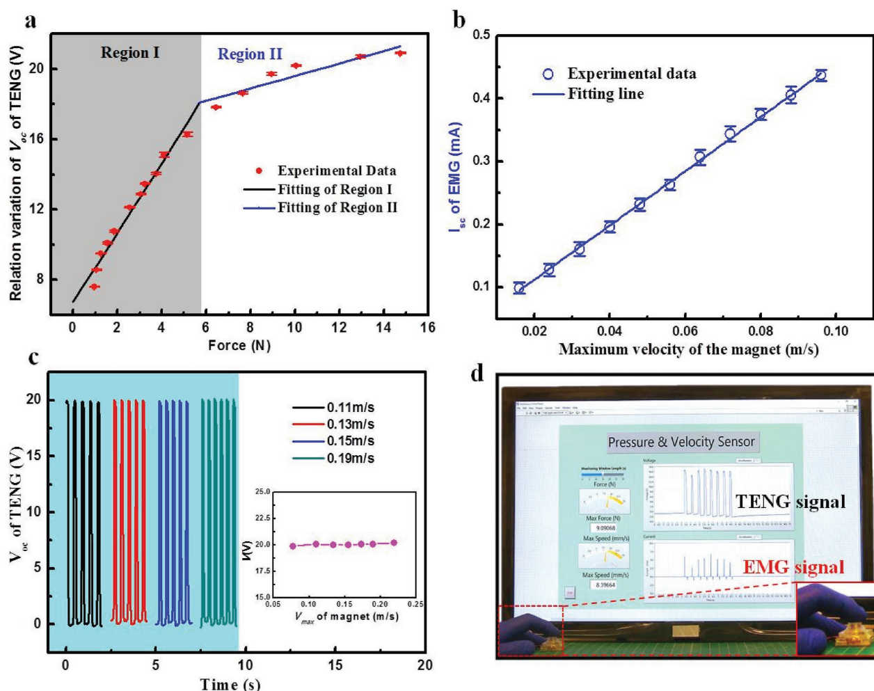
Figure 5. Electrical output performance of the EMG-TENG active sensor. a) The relative variation of the V_{oc} of the TENG part versus different external forces applied on the TENG. b) The short-circuit current of the EMG part versus the maximum velocity of the magnet. c) The open-circuit voltage of TENG versus time under different maximal velocity of magnet and same external force. The inset shows the relationship between the open-circuit voltage and the maximal velocity of magnet. d) Demonstration of the ETAS for recording the press force and velocity from keystroke.
