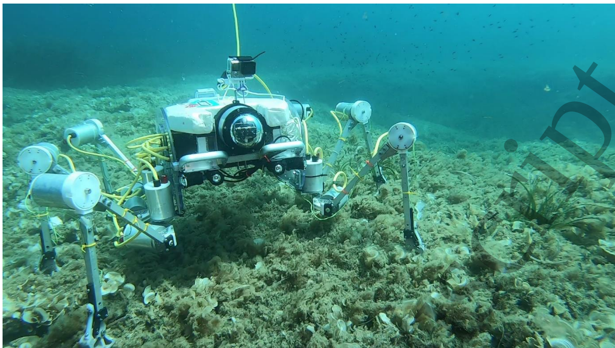
Figure 2. SILVER2 robot.
