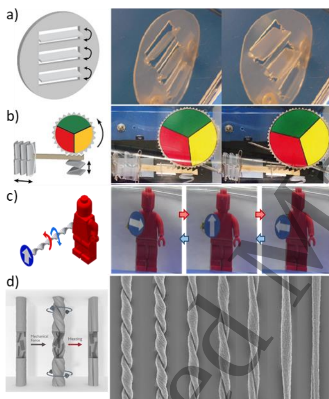
Figure 2. a) SMPA based shading lamellas b) heat engine driven by a concertina-shaped SMPA drive element (a, b adapted with permission from [3]). c) Reversible noncontinuous twisting actuation (adapted with permission from [17], copyright 2017 American Chemical Society). d) SMP fibers for rotating microengines. (figure on the right: adapted with permission of the American Association for the Advancement of Science from [12], permission conveyed through Copyright Clearance Center, Inc.).
