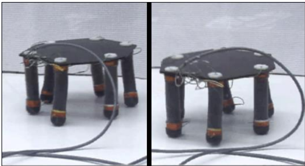
Figure 2. Example of a bioinspired robot using dielectric elastomers both as structural components (legs) and actuators (muscles). Imaged adapted from [12]
