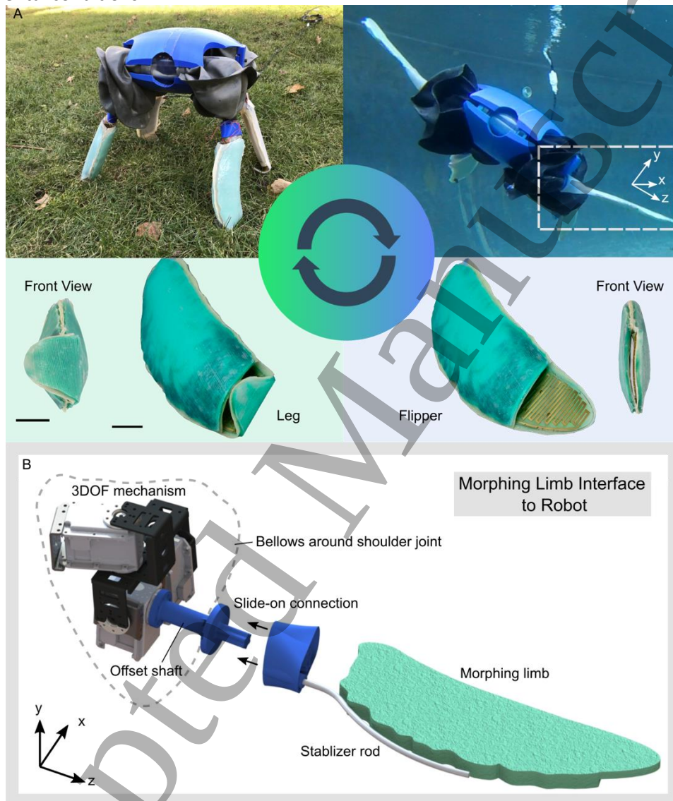
Figure 3. A. Morphing limbs attached to a quadruped turtle-inspired robot allow it to engage in swimming and walking. The morphing limb is able to switch between flipper and leg shape using variable stiffness materials and fluidic elastomer actuator (limb images adapted from [8]). B. Schematic showing how a morphing limb interfaces to the kinematic mechanism within the waterproof bellows.
