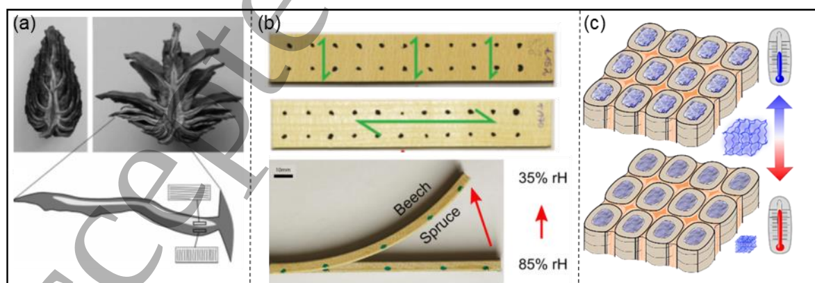
Figure 1. (a) A pine cone cut along its longitudinal axis, with one half wet and one half dry (mirrored in the image); drawing of the bilayer structure of the scale and the cellulose fibril orientations in the cell walls [1] reprinted with permission of The Royal Soc.; (b) Bioinspired wooden bilayer with different fibre orientation actuated by humidity change [2]; (c) in situ formation of PNIPAM hydrogel in the lumina of wood cells for wood materials with embedded temperature responsivity [7] reprinted with permission of Wiley.
