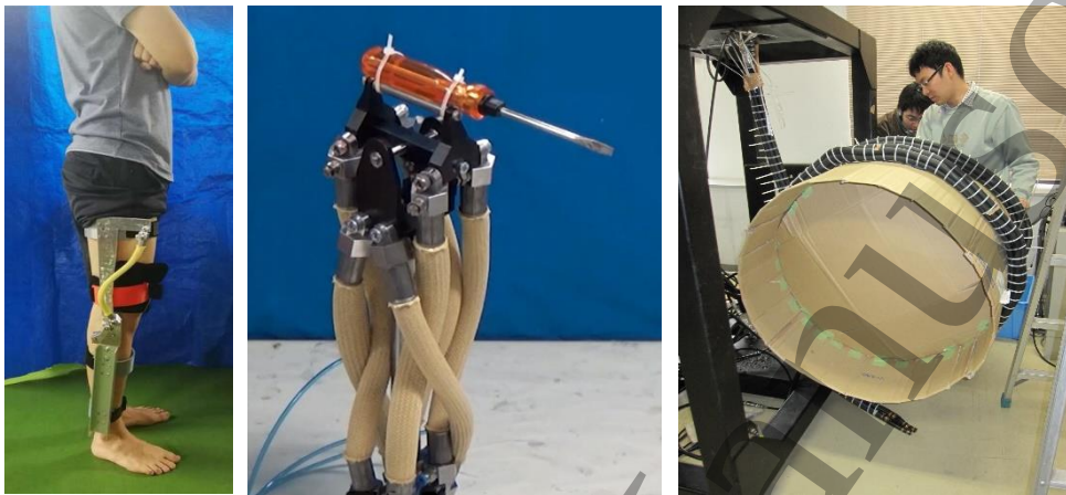
Figure 2. Examples of power soft robot applications of soft hydraulic muscles. Knee support device based on four-bar linkage and hydraulic artificial muscle [12] (left), rotational-compliant joint with hydraulic McKibben artificial muscles [13] (middle), and long bending rubber arm combining contracting and extending muscles [14] (right).
