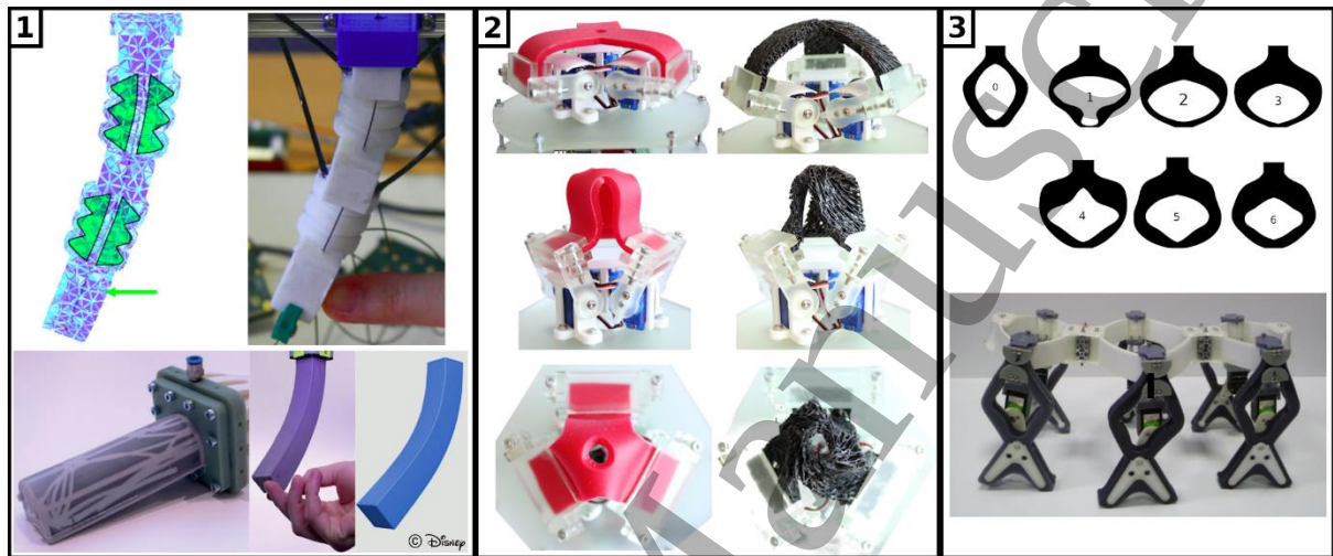
Figure 2. 1| top : Sensor Fusion Approach for Force and Shape Estimation using FEM [6], bottom : Sensor Design for Proprioceptive Soft Robots [5] 2| Simulation and use of mesostructured material to create anisotropic behavior [10] 3| use of an evolutionary optimization algorithm to do shape optimization [11].
